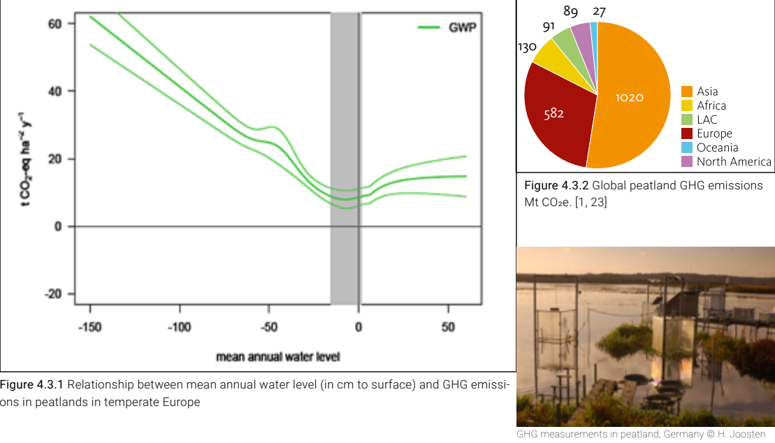
GHG measurements in peatland, Germany © H. Joosten
