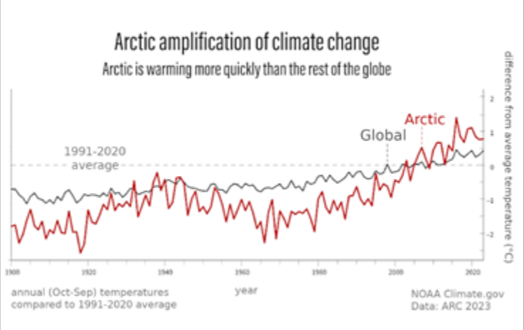
Figure 2.2.2 Temperature rise globally and in the arctic zone [28]
