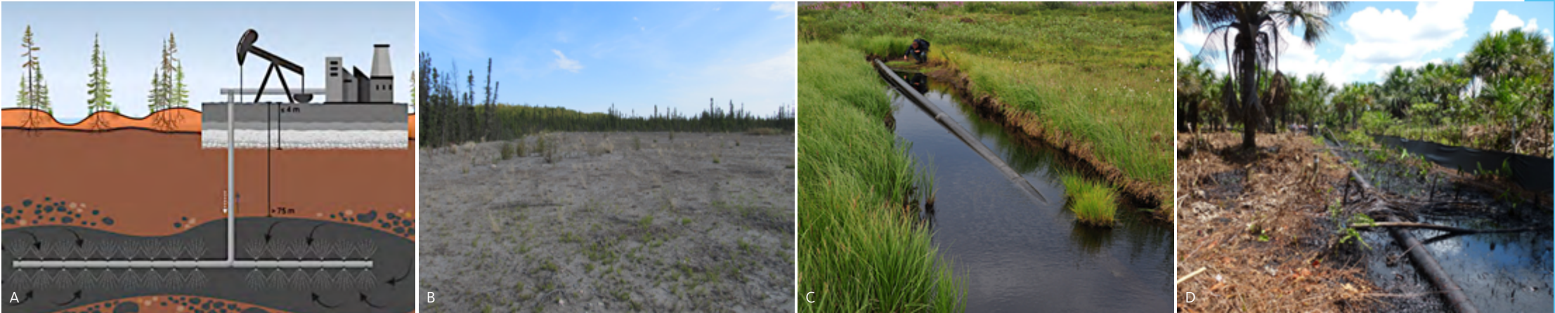
Figure 4.7.2 Extraction infrastructure and pipe lines on peatlands: A) scheme of an in-situ oil pad built on peatland (Canada [1]); B) foundation of a oil pad on peatland (Canada); C) gas pipeline on peatland in Russian Arctic; D) oil infrastructure and contamination in wetland/peatland of the Pastaz-Marañón Basin in Peru.
