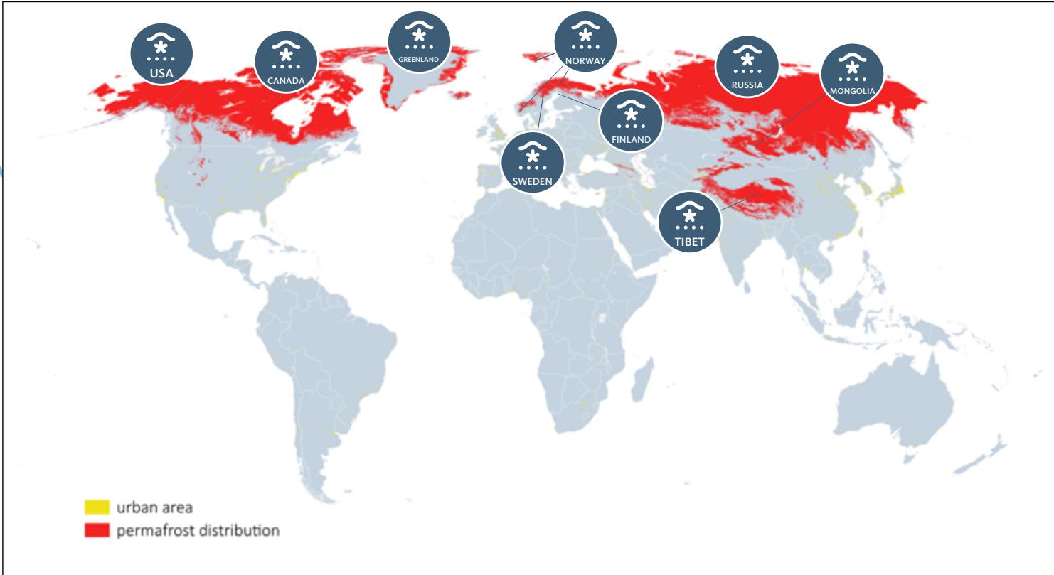
Map 2.2.1 World permafrost distribution [28]
