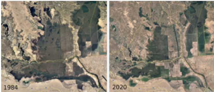
Figure 2.4.2 Wetland loss in the Hammar marshes (Iraq) from 1984-2020 due to drainage, dam construction, and agriculture (Satellite images by Google Earth).
